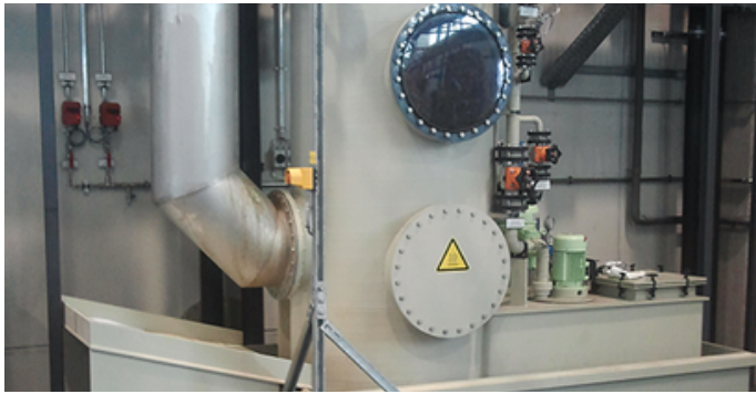
Dedusting system Dry/Wet
