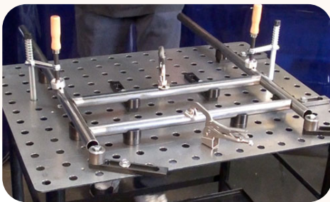
Welding table
