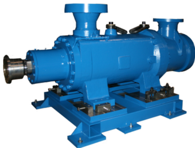
Three Screw Crude Oil Pump
