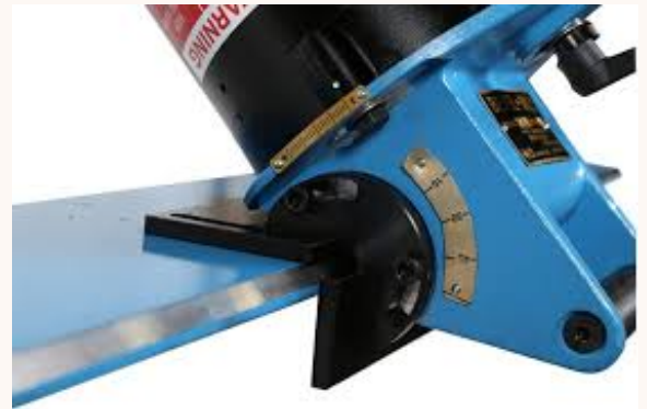
Plate Beveller
