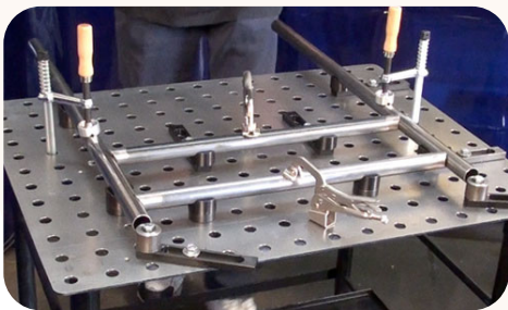
Welding table
