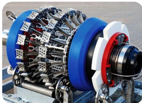
Smart pig
