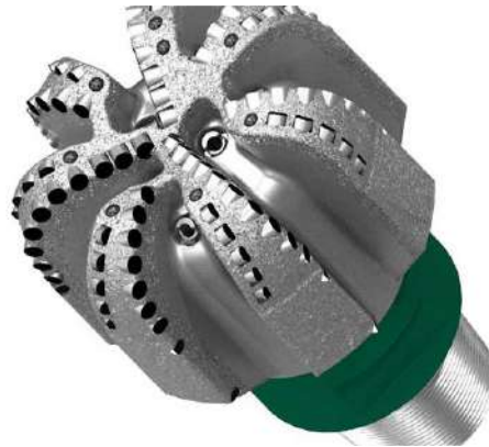
PDC bit
