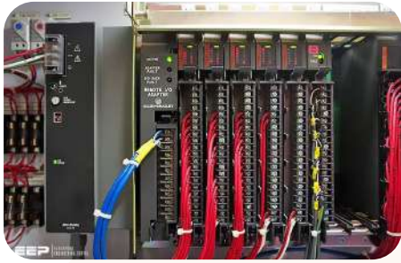
RTU/SCADA systems
