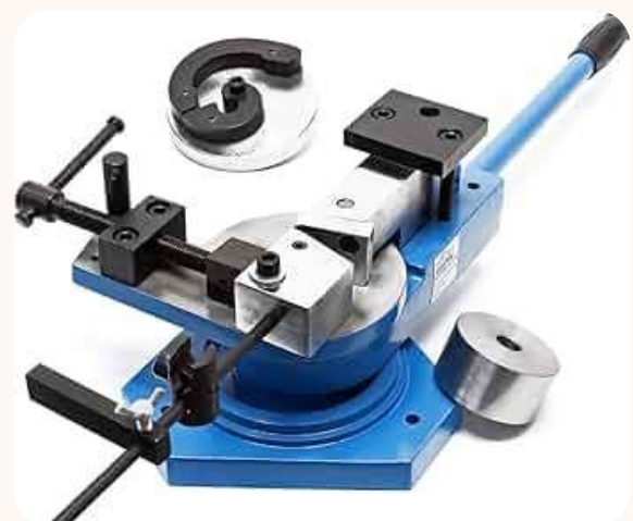
Bending machine
