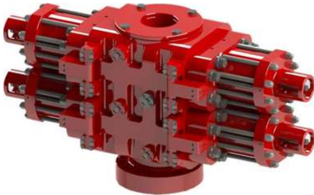
RAM type BOP
