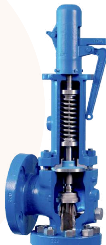
Pressure relief valve
