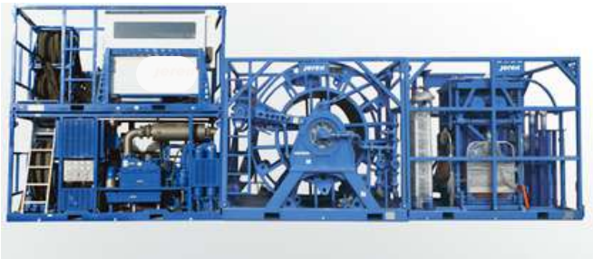
Skid mounted coiled Tubing Unit
